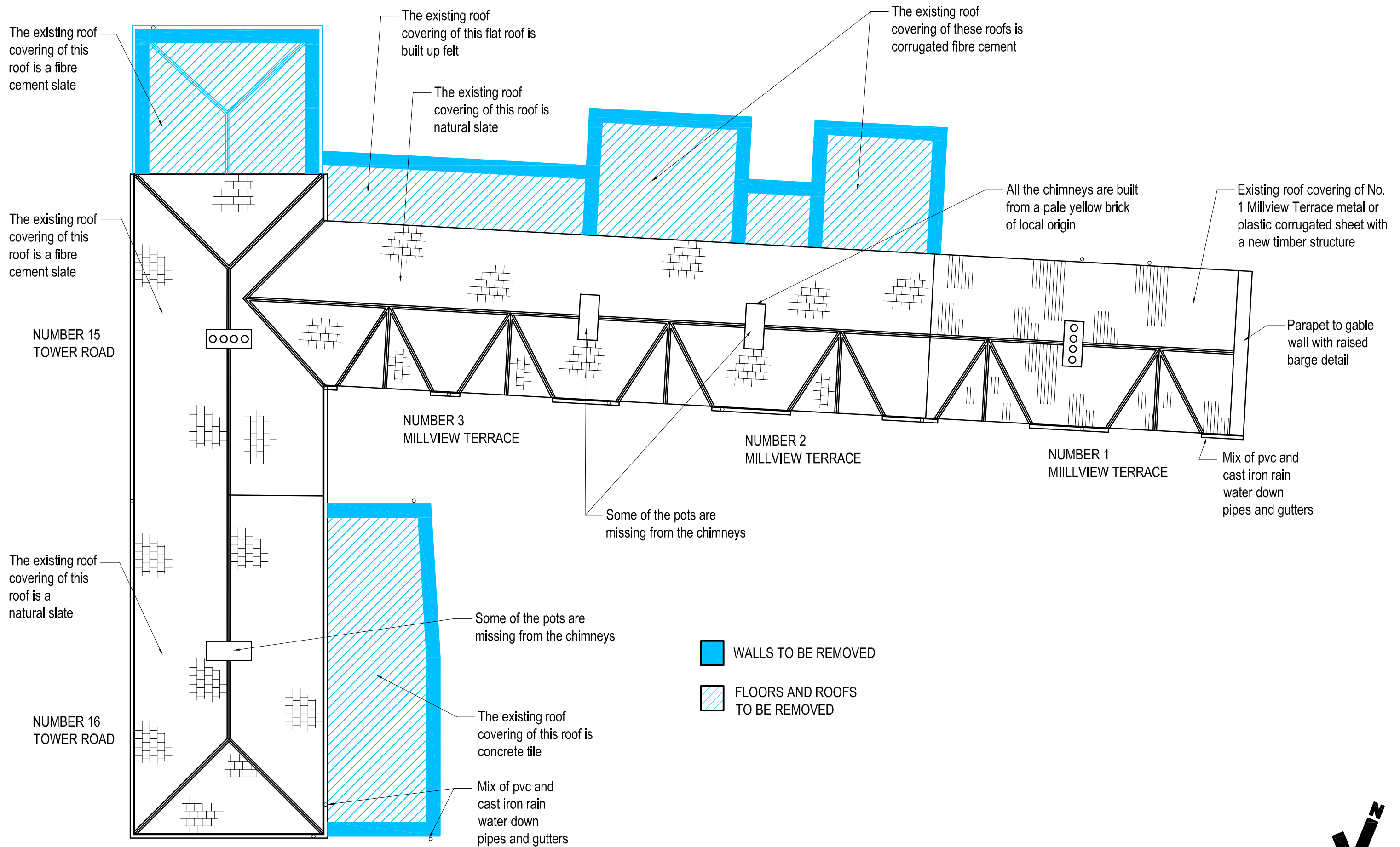
07 EXISTING ROOF PLAN SCALE = 1:100 @ A3
