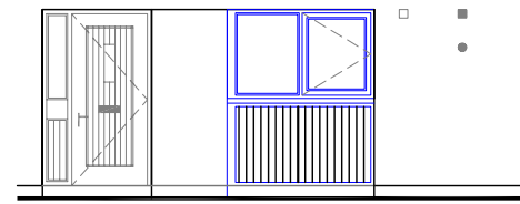
FRONT ELEVATION - K4
