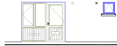
REAR ELEVATION - K4
