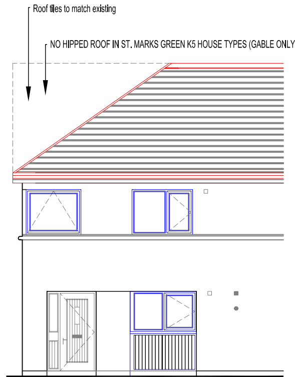
FRONT ELEVATION - K5 (GABLE)
