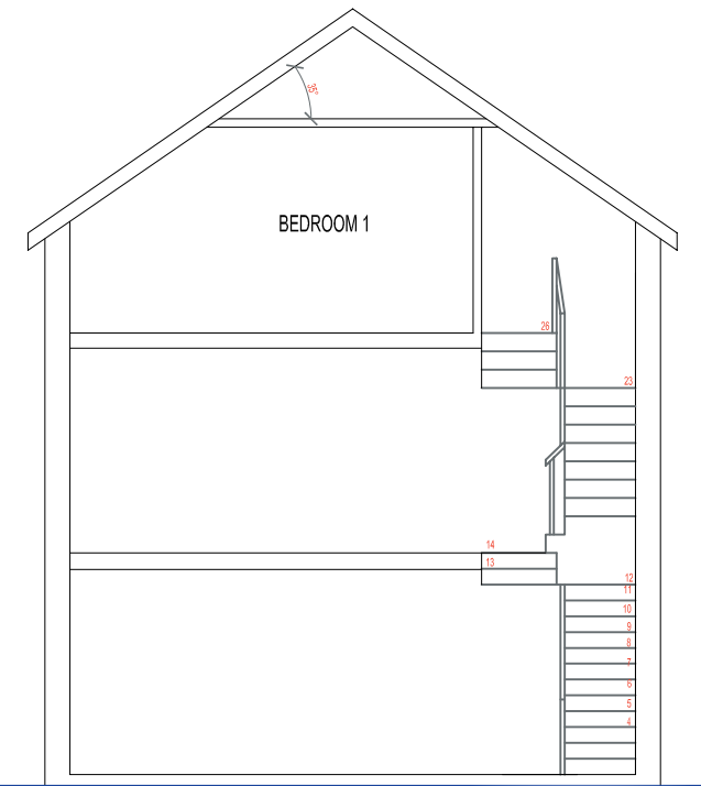
TYPICAL SECTION
