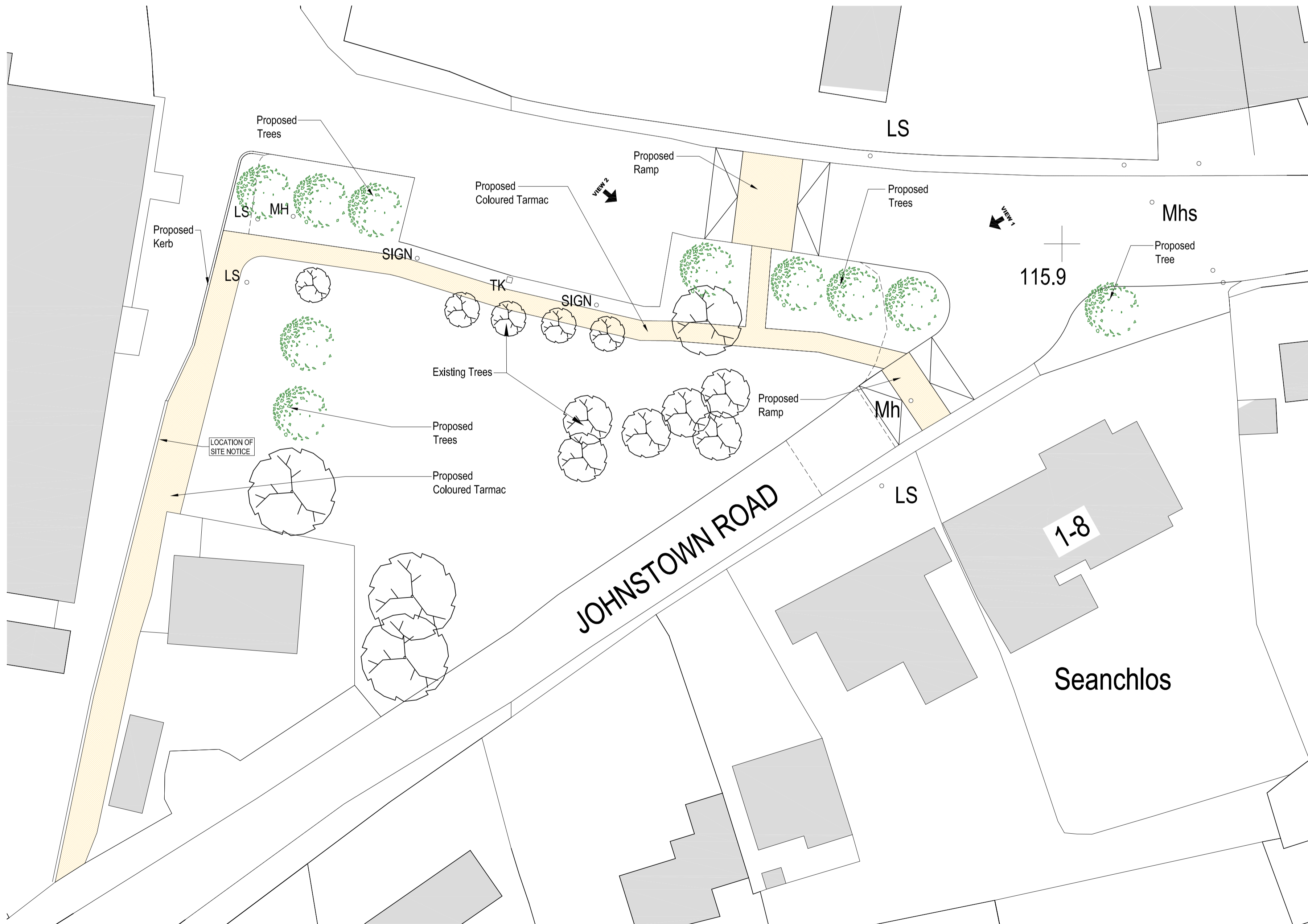
01 VILLAGE GREEN PROJECT PLAN P8 1:250
