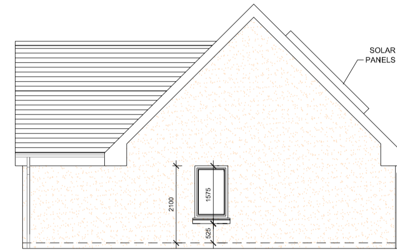
SIDE ELEVATION
