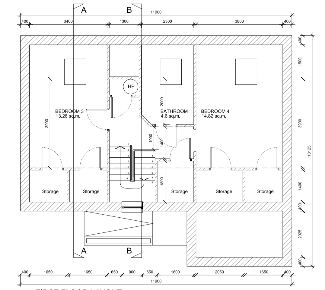
FIRST FLOOR LAYOUT
