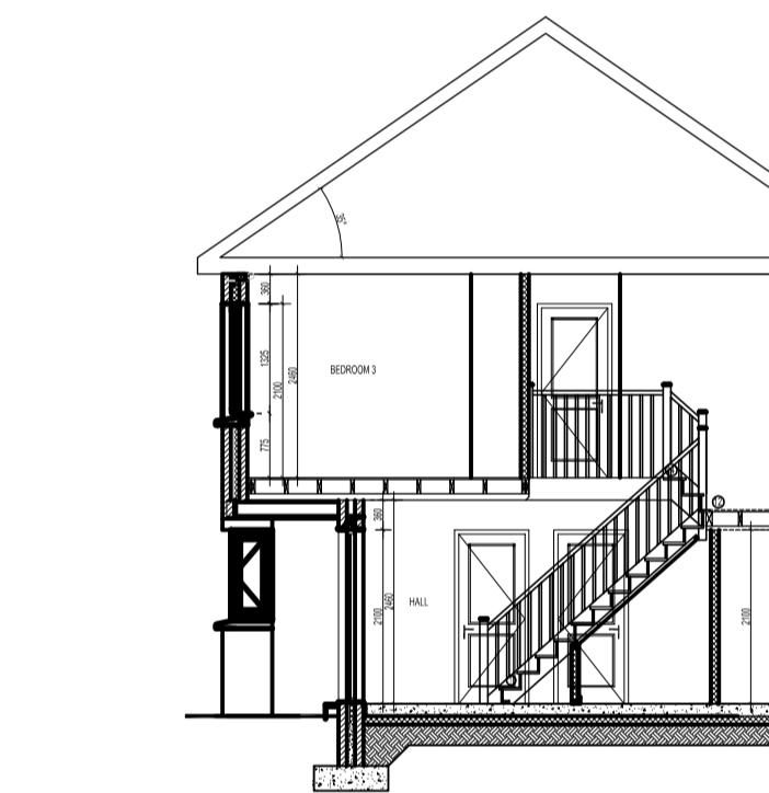
HOUSE TYPE K5- SECTION A-A 1:100
