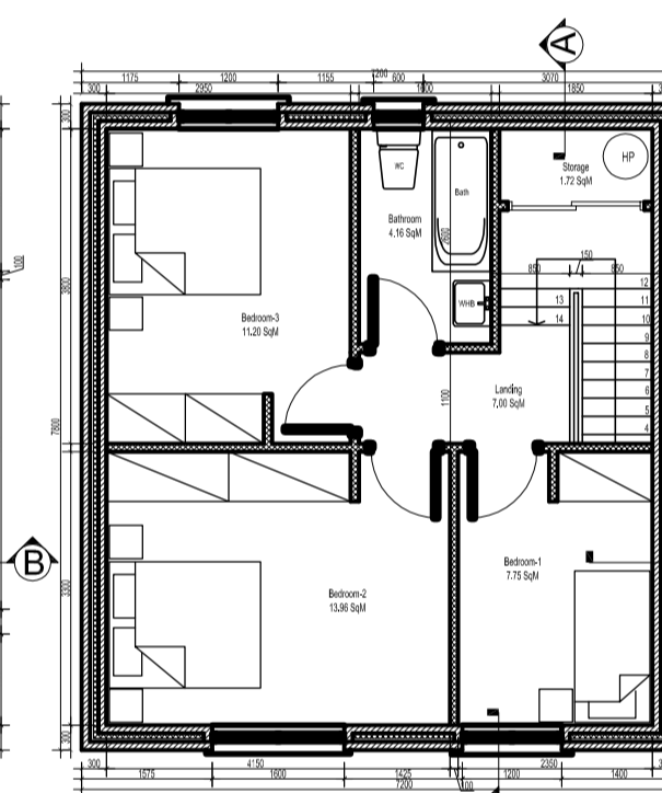
HOUSE TYPE K5- FF PLAN 1:100
