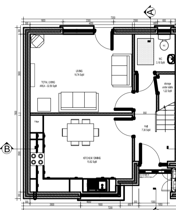
HOUSE TYPE K5- GF PLAN 1:100
