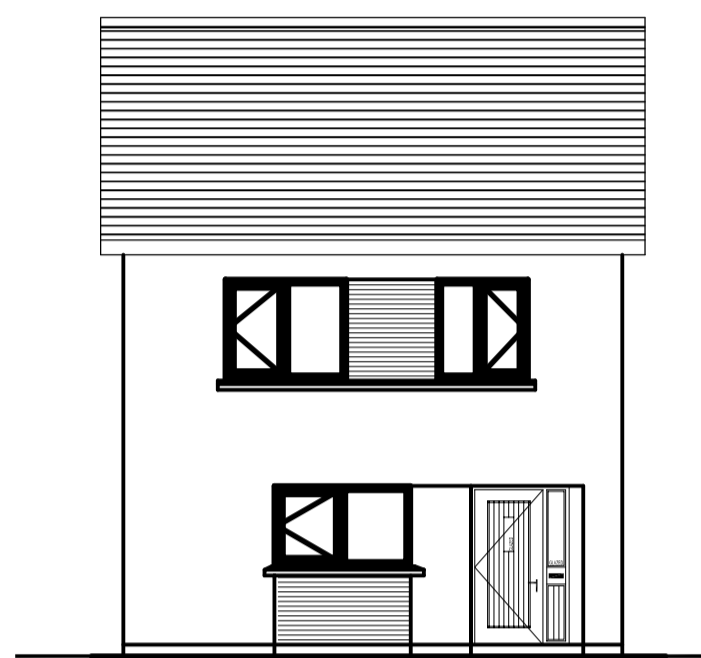
HOUSE TYPE K4- FRONT ELEVATION 1:100
