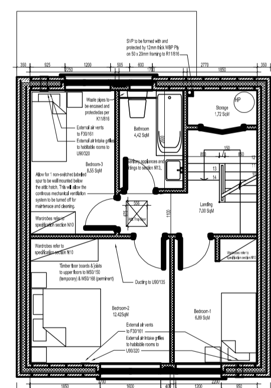
HOUSE TYPE K6- 1F PLAN 1:100
