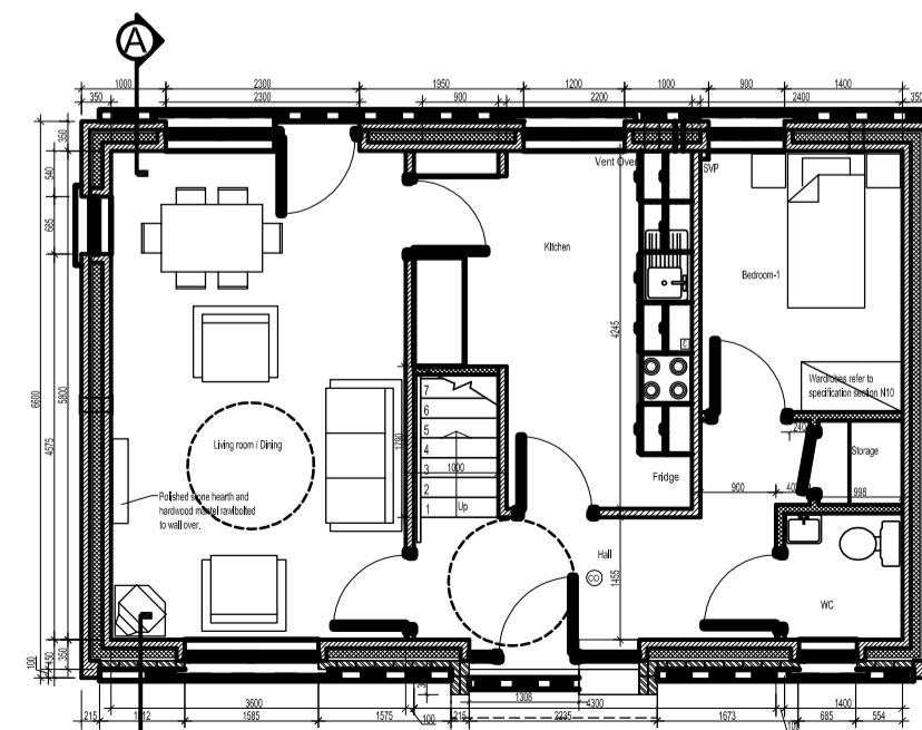
HOUSE TYPE L5- GF PLAN 1:100
