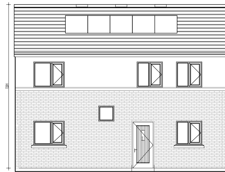
HOUSE TYPE C5- FRONT ELEVATION 1:100
