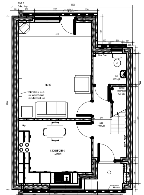
HOUSE TYPE K6- GF PLAN 1:100
