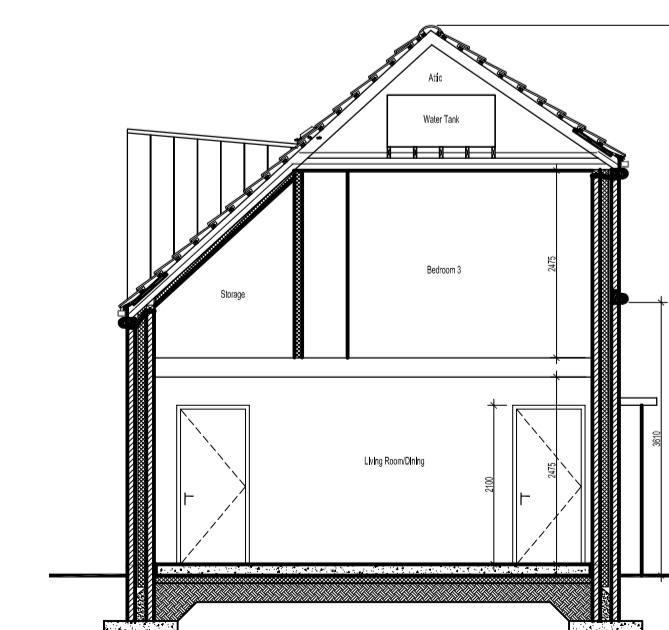
HOUSE TYPE L5- SECTION A-A 1:100
