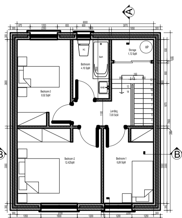
HOUSE TYPE K4- FF PLAN 1:100
