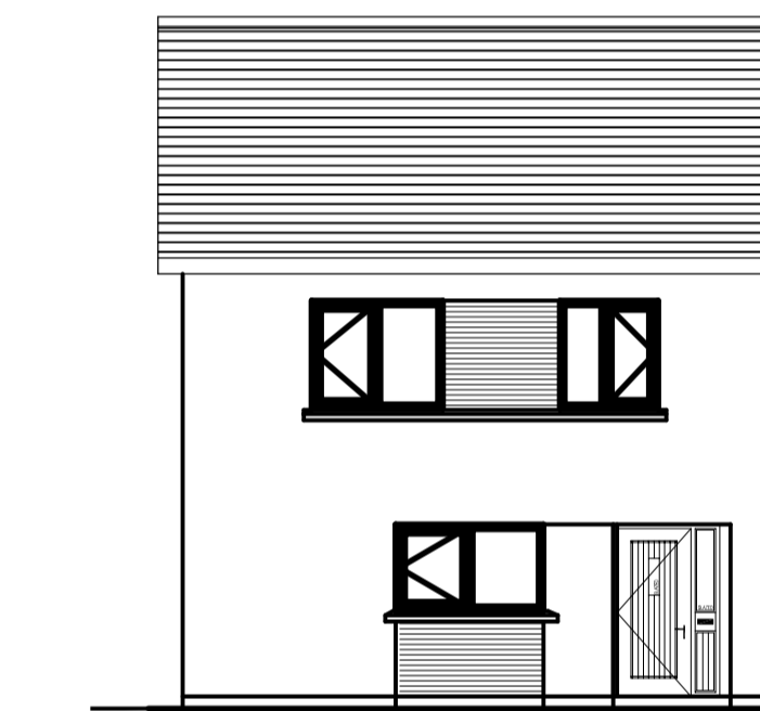
HOUSE TYPE K5- FRONT ELEVATION 1:100
