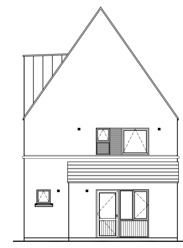
HOUSE TYPE K6- REAR ELEVATION 1:100
