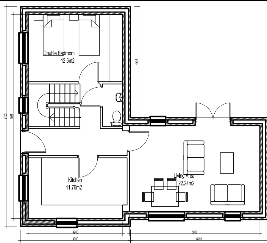
HOUSE TYPE C5- GF PLAN 1:100
