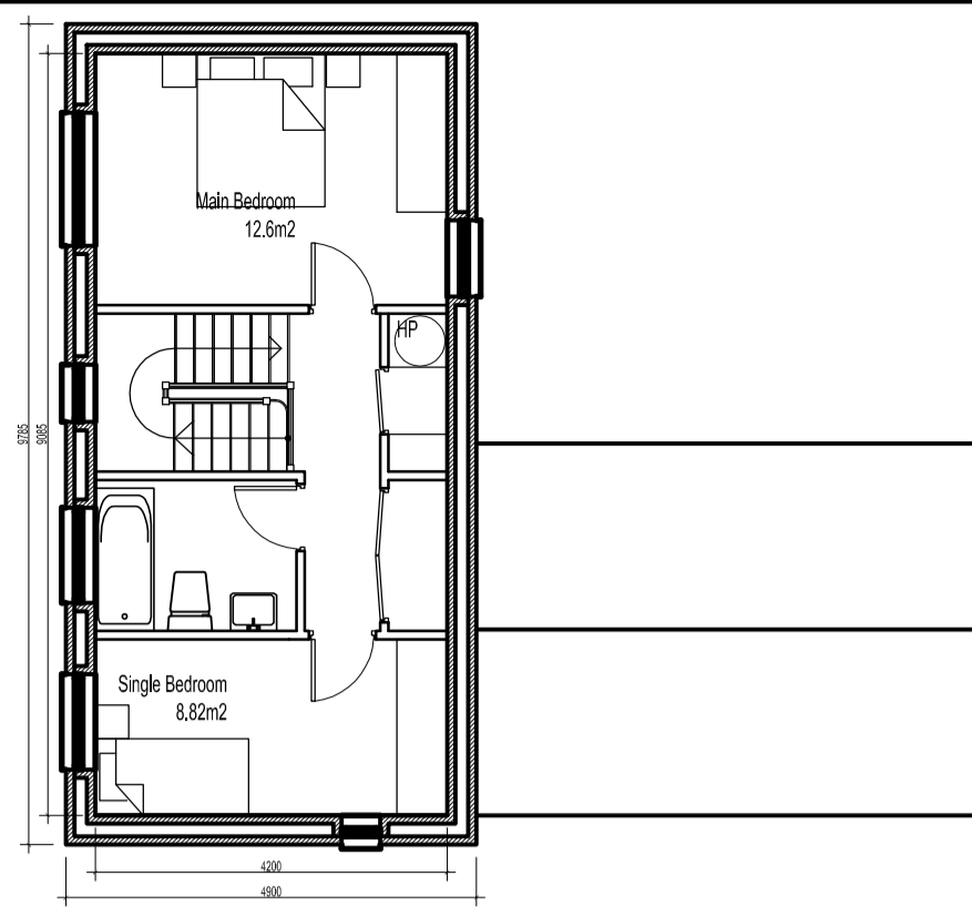
HOUSE TYPE C5- FF PLAN 1:100
