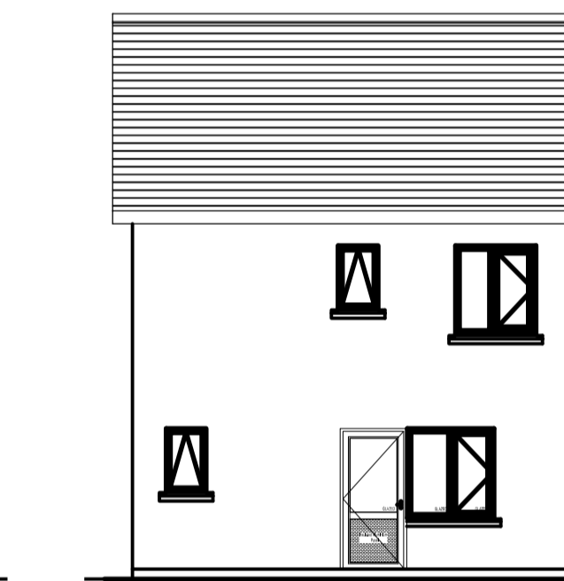
HOUSE TYPE K5- REAR ELEVATION 1:100
