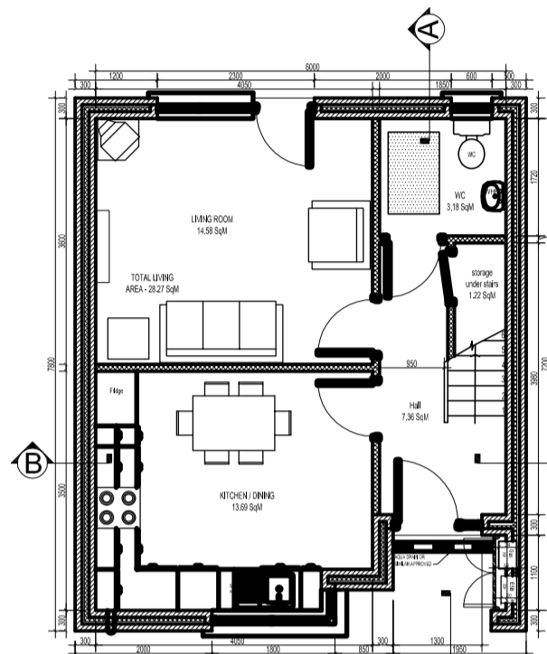
HOUSE TYPE K4- GF PLAN 1:100
