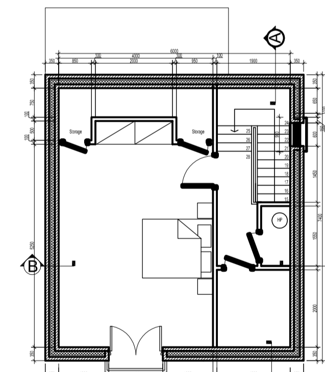
HOUSE TYPE K6- 2F PLAN 1:100
