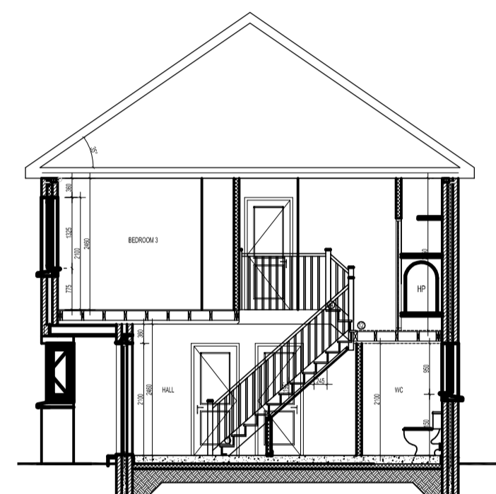
HOUSE TYPE K4- SECTION A-A 1:100
