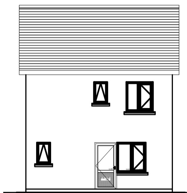
HOUSE TYPE K4- REAR ELEVATION 1:100
