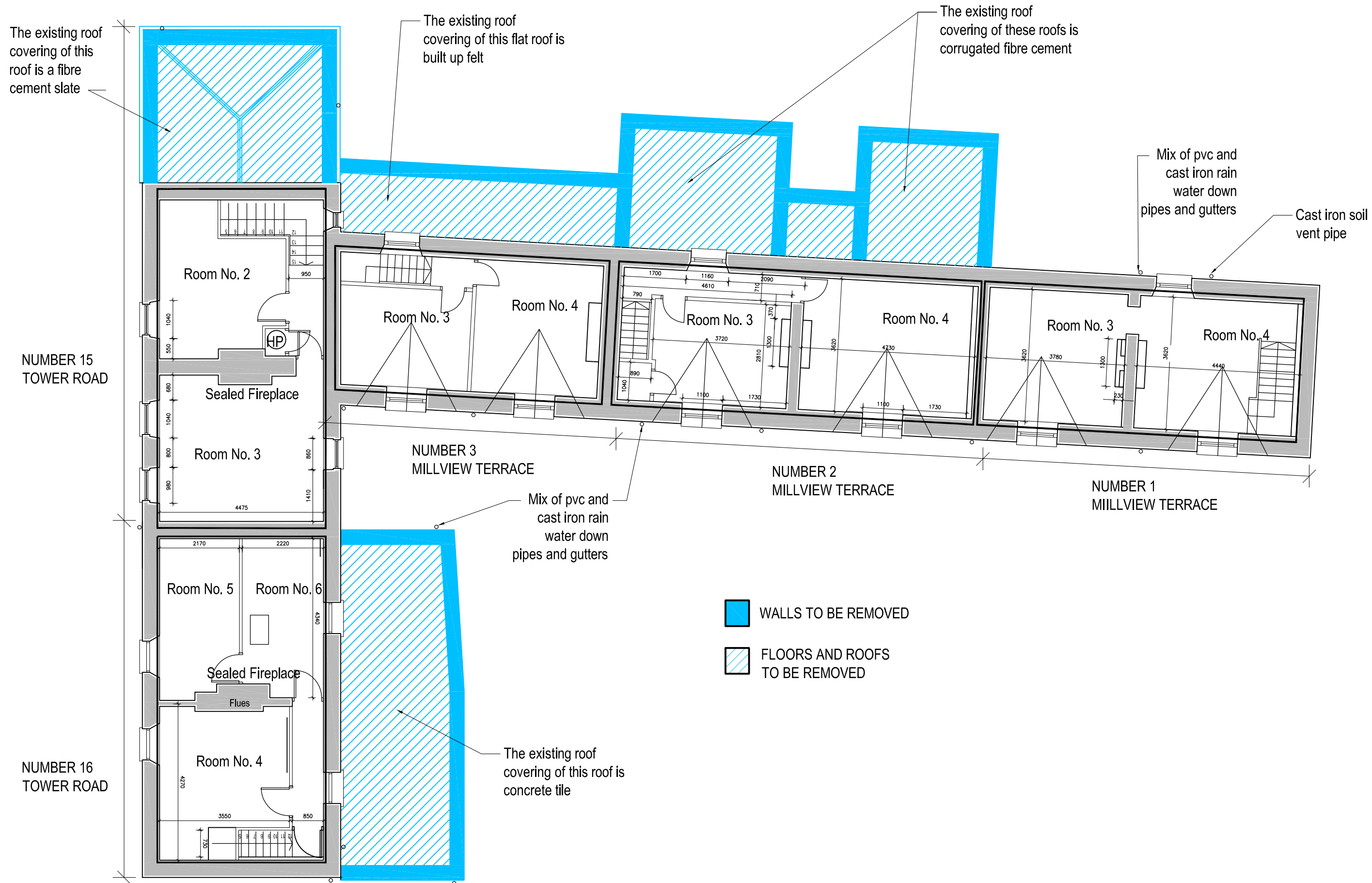
06 EXISTING FIRST FLOOR PLAN SCALE = 1:100 @ A3
