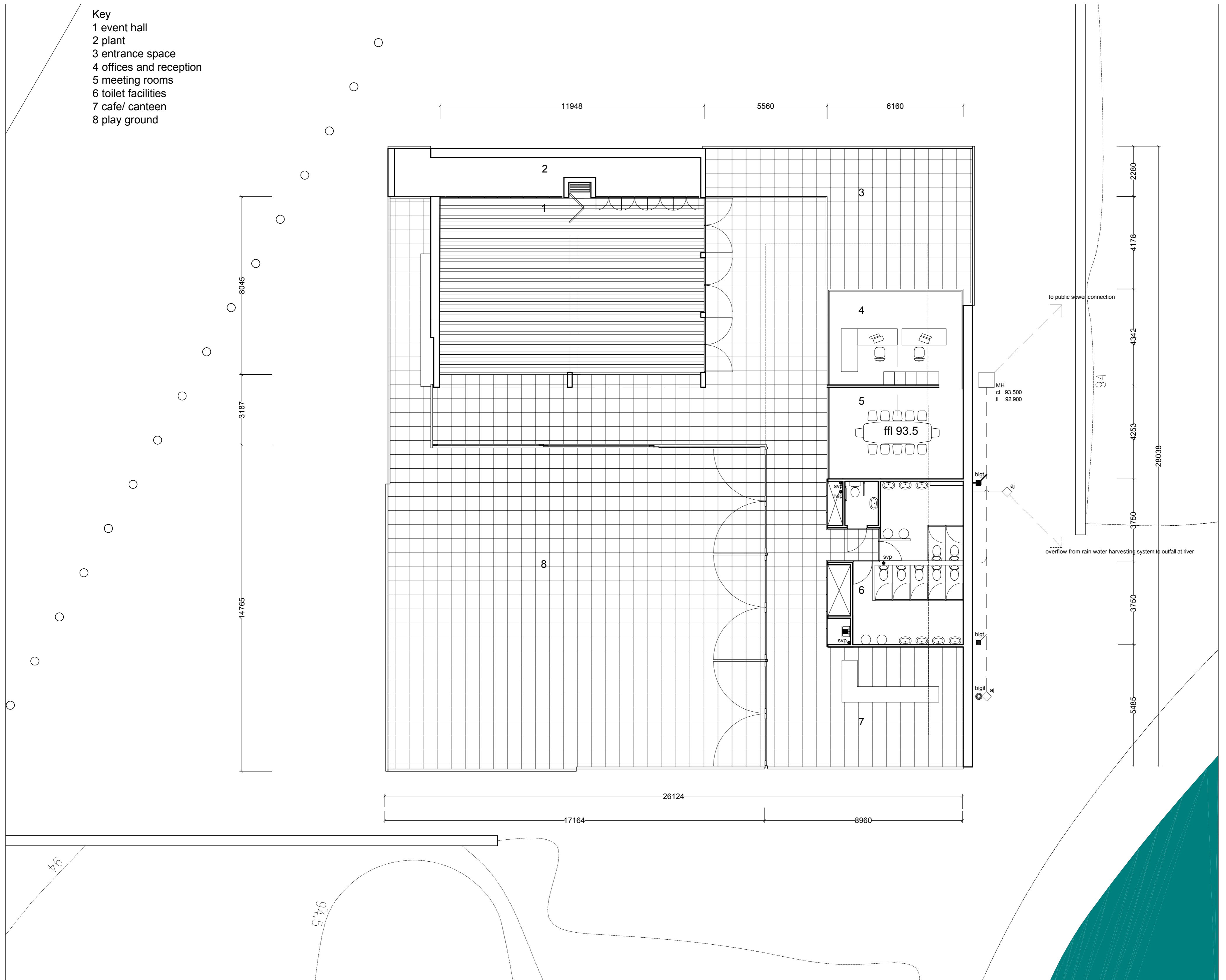
floor plan 1:100
